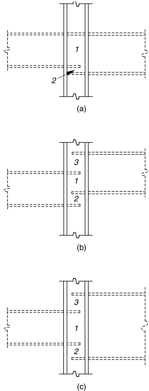
Figure 5-1 Columns with beams of differing depths and/or tops of steel.
