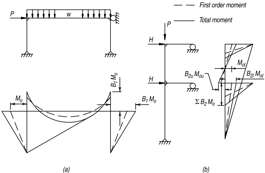
Fig. C-C1.1. Moment amplification.
