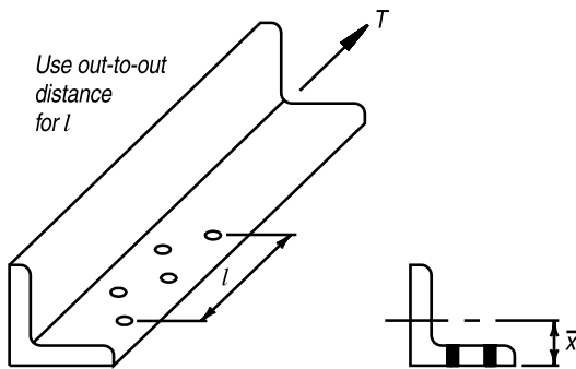
Fig. C-B3.2. Staggered holes.
