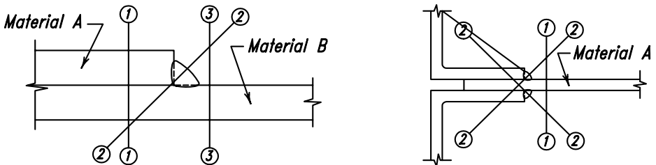
Fig. C-J2.10. Shear planes for fillet welds loaded in longitudinal shear.
