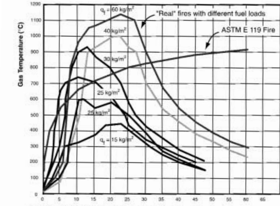
Figure 28. Time/temperature curves for various fire exposures
