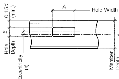
ECCENTRIC WEB PENETRATION
