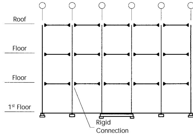
Figure 12. Rigid frame building elevation
