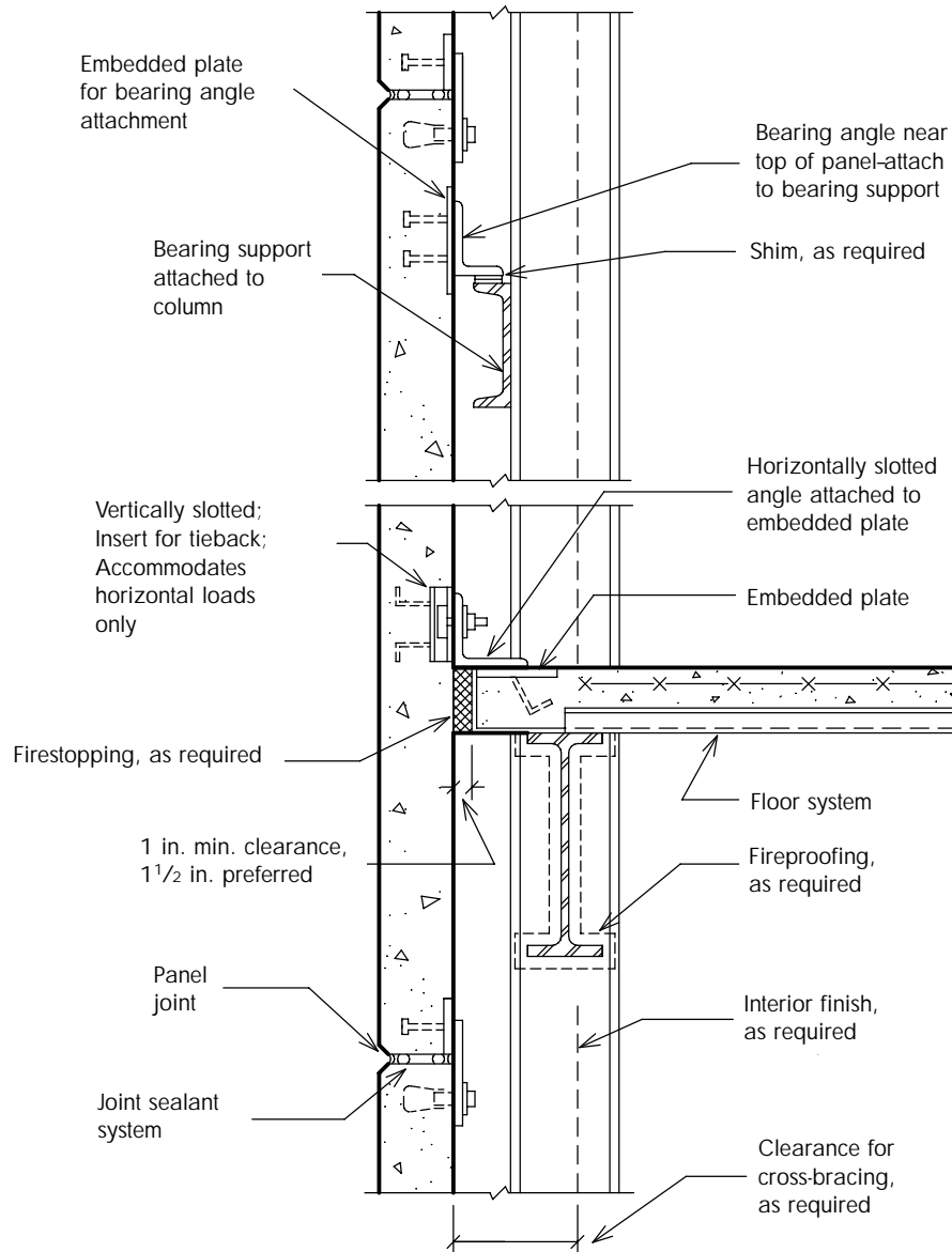
Figure 2b. Detailing Considerations for Precast Concrete Panels (Sample Wall Section Detail at Horizontal Span Precast Panels)
